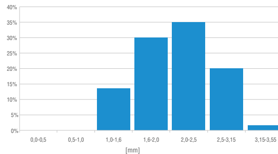
SIEVE ANALYSIS 1,0 - 3,0 mm
